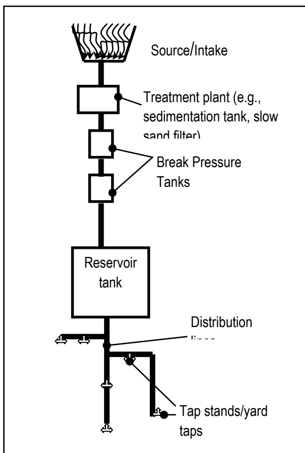
Figure 6. 9: Schematic diagram of a Gravity Flow Scheme
