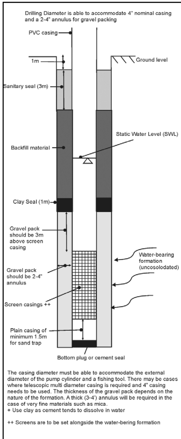
Figure 6. 2: Drilled well design (shallow well design) for both shallow and deep wells in unconsolidated formation
