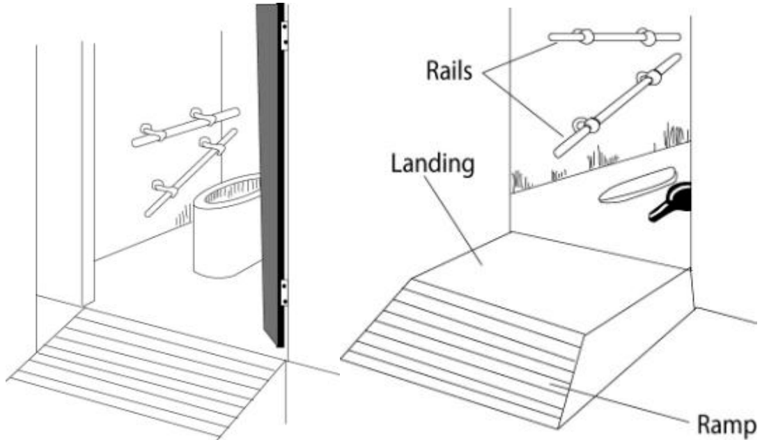
Figure 6. 16: Sanitation structures for persons with disabilities: left- pit latrine fitted with hand support and a pedestal and right- pit latrine fitted with a landing, rails for hand support and a squat hole
