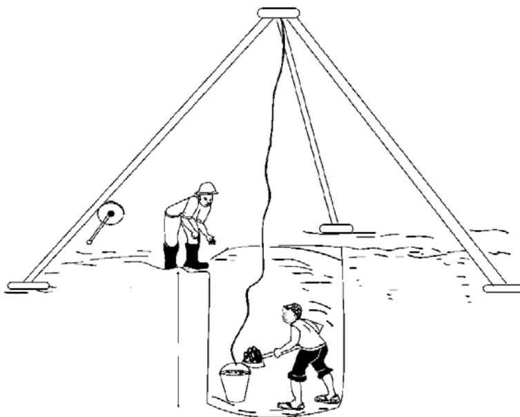
Figure 6. 1: Construction of hand dug well
