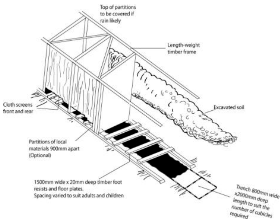
Figure 6.17: Trench Latrines
