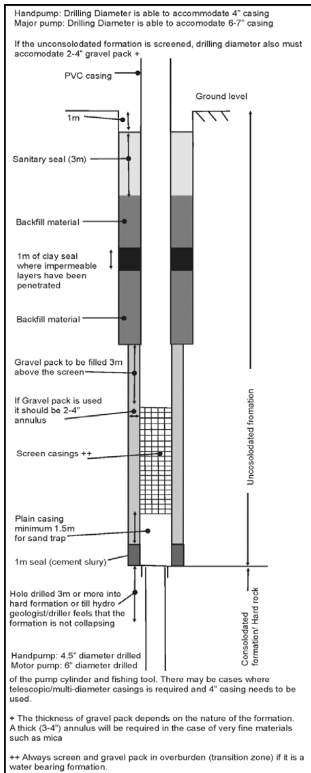
Figure 6. 3: Drilled well design for consolidated formation/hard rock (open hole design)
