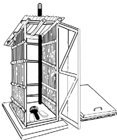
Figure 6.15: Fossa alterna toilet (source IRC, SNV and Netwas publication)
